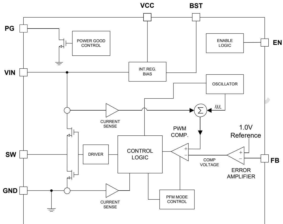
Fig.3 Functional Diagram
