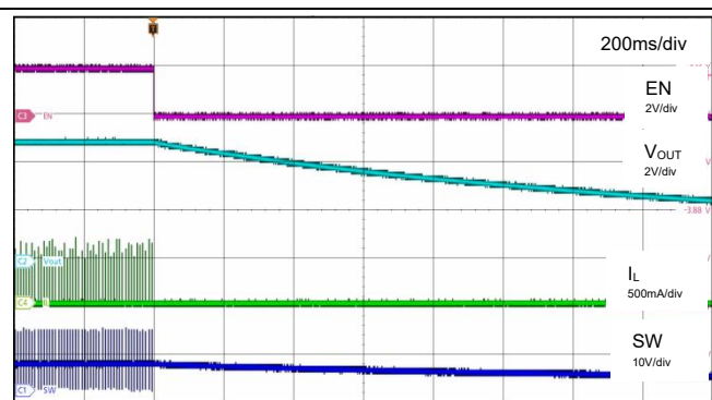
Fig.22 Shutdown through EN at I_{LOAD}=0A
