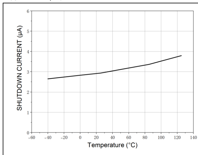
Fig.4 Shutdown Current vs. Junction Temperature
