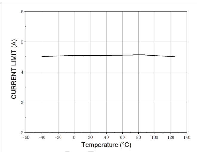
Fig.5 Current Limit vs. Junction Temperature at Duty = 40%
