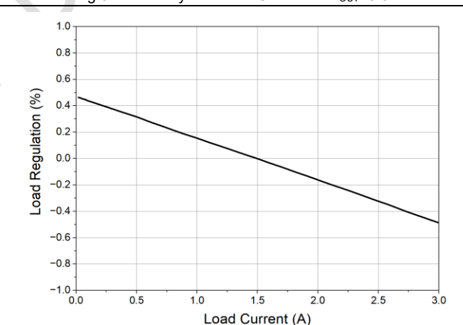
Fig.34 Load Regulation VS. Load Current at V_{IN}=12V
