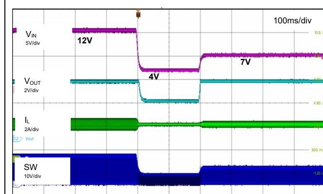
Fig.31 Cold-Crank at V_{OUT}=5V , I_{OUT}=3A
