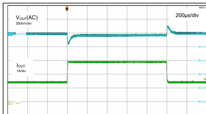
Fig.29 Load Transient at I_{LOAD} from 1.5A to 3A, 1.6A/μs
