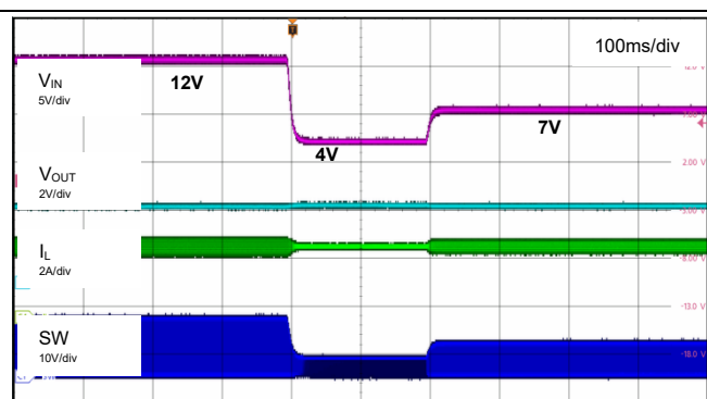
Fig.30 Cold-Crank at V_{OUT}=3.3V , I_{OUT}=3A
