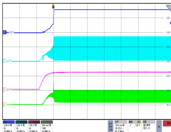
Figure 11. Power On by V_{IN} V_{IN}=1.2V , V_{OUT}=3.3V , I_{OUT}=90mA
