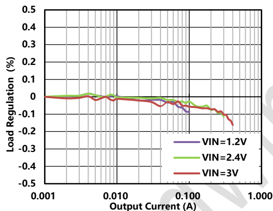
Figure 5. Load Regulation ( V_{OUT}=3.3V )
