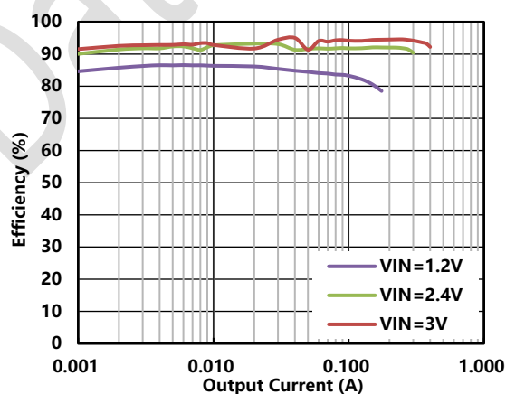
Figure 6. Efficiency vs. Output Current ( V_{OUT}=3.3V )
