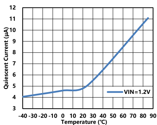
Figure 8. Quiescent current vs. Temperature ( V_{OUT}=3.3V )
