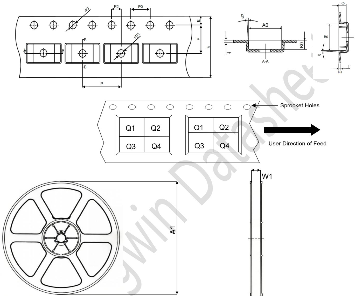
Figure 25. TAPE and Reel Information
