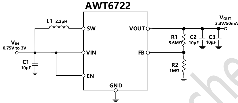
Figure 21. Typical Application Circuit
