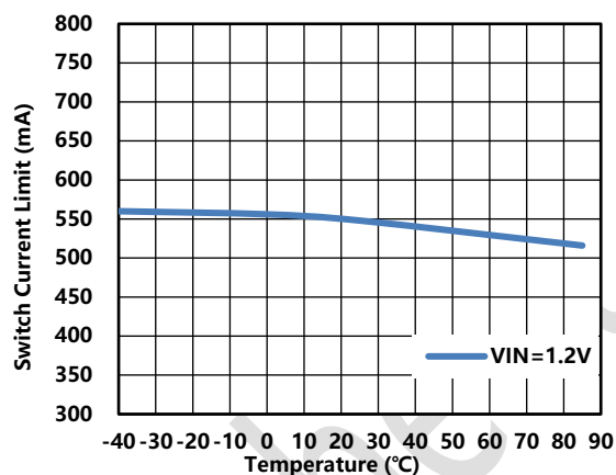
Figure 10. Switch Current Limit vs. Temperature ( V_{OUT}=3.3V )
