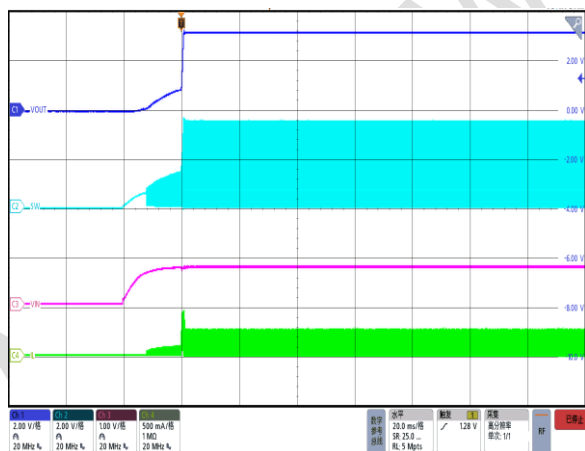
Figure 13. Power On by V_{IN} V_{IN}=0.75V , V_{OUT}=3.3V , I_{OUT}=5mA
