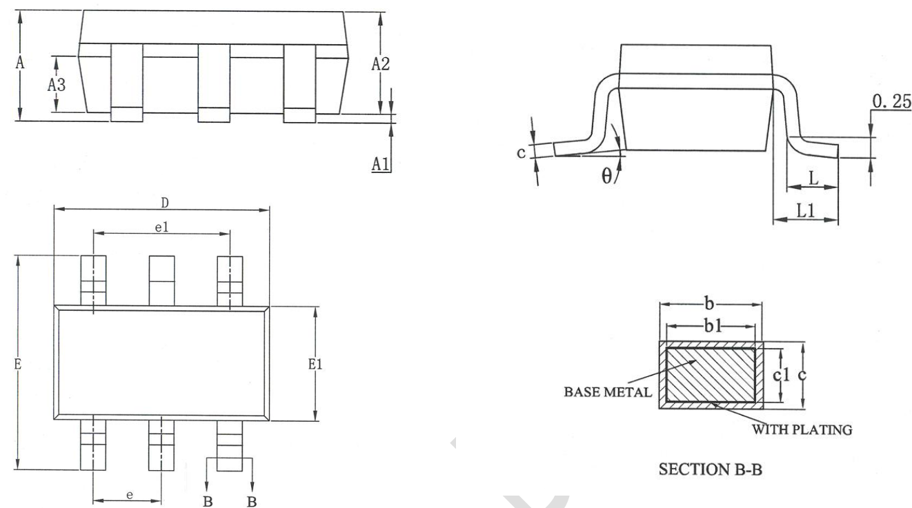
Figure 26. SOT23-6 Package
