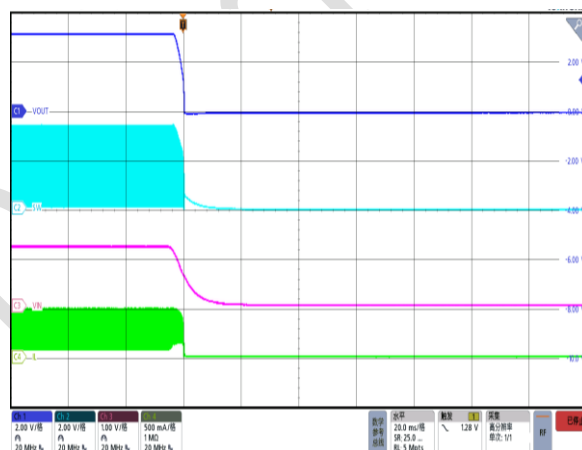
Figure 12. Power Off by V_{IN} V_{IN}=1.2V , V_{OUT}=3.3V , I_{OUT}=90mA
