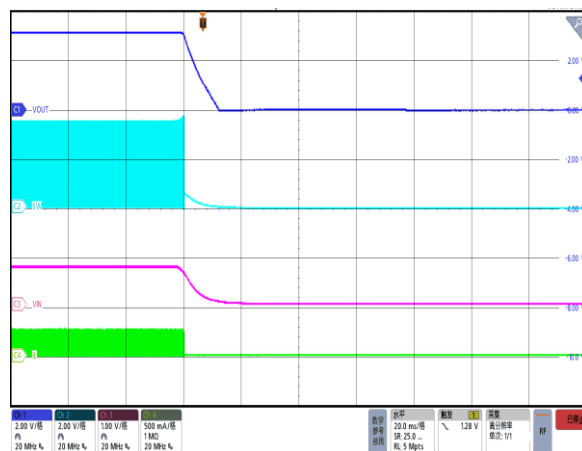
Figure 14. Power Off by V_{IN} V_{IN}=0.75V , V_{OUT}=3.3V , I_{OUT}=5mA
