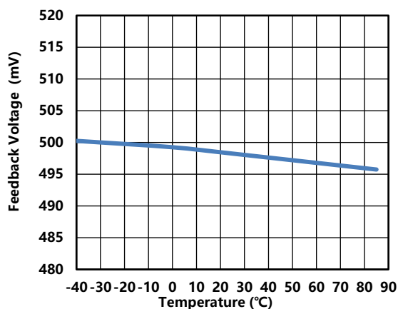
Figure 9. Feedback Voltage vs. Temperature ( V_{OUT}=3.3V )
