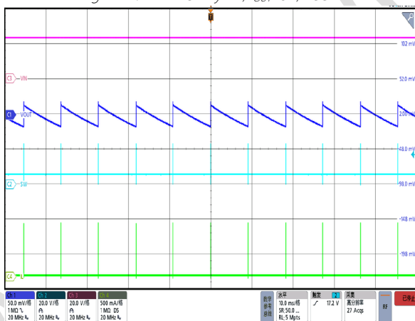
Figure 43. Switching Waveform, I_{OUT}=0A , PFM
