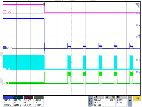
Figure 48. SCP Entry, I_{OUT}=0A , FCCM
