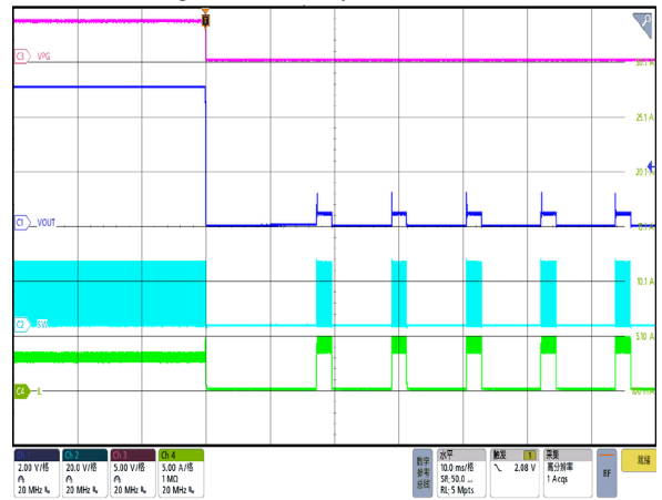
Figure 50. SCP Entry, I_{OUT}=3A , FCCM
