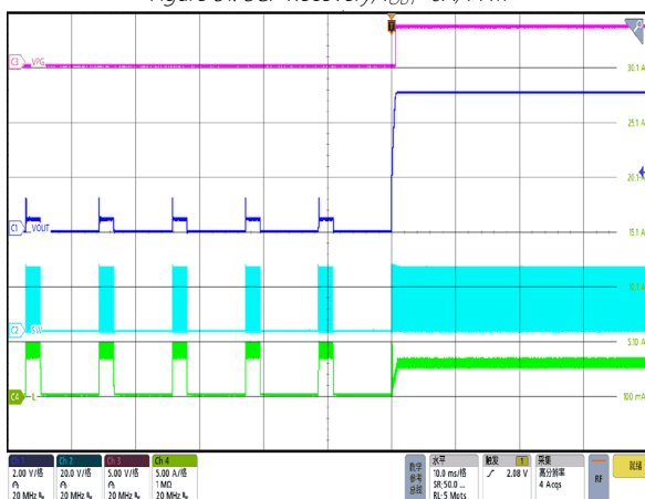
Figure 53. SCP Recovery, I_{OUT}=3A , PFM
