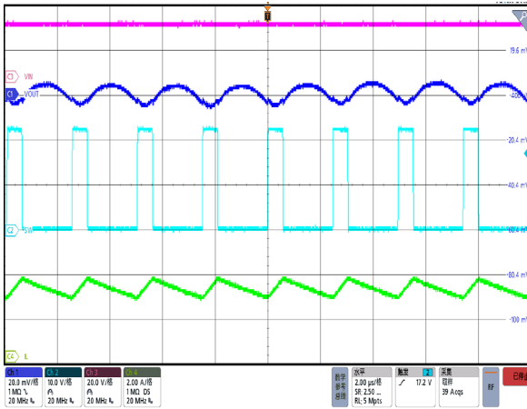
Figure 45. Switching Waveform, I_{OUT}=3A , PFM
