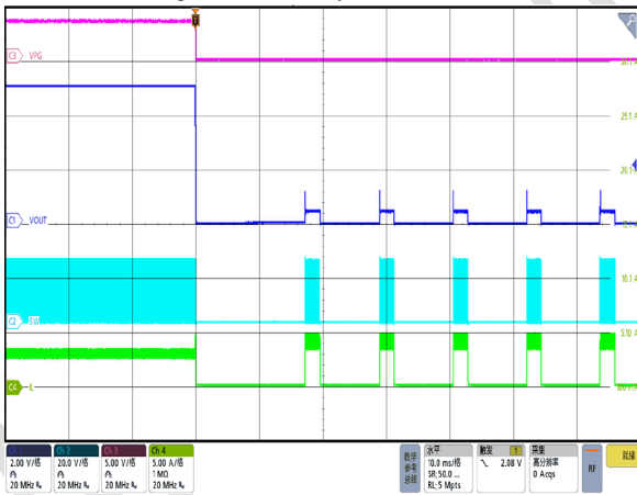
Figure 49. SCP Entry, I_{OUT}=3A , PFM
