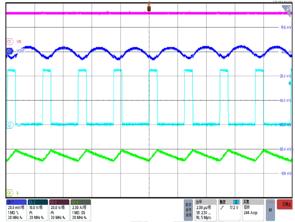
Figure 46. Switching Waveform, I_{OUT}=3A , FCCM
