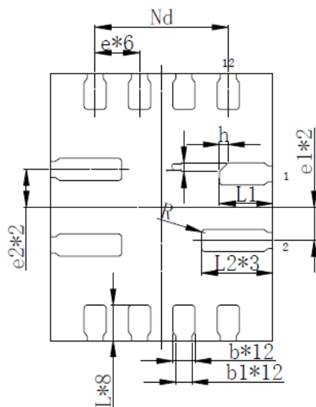
BOTTOM VIEW
