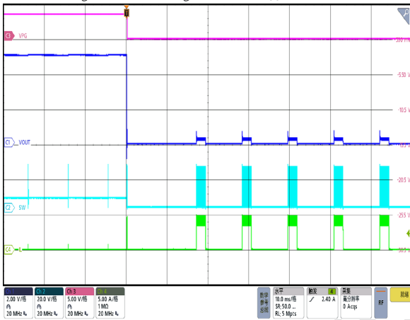
Figure 47. SCP Entry, I_{OUT}=0A , PFM
