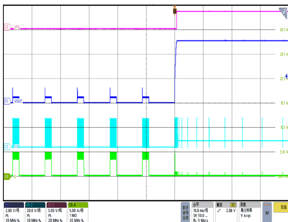
Figure 51. SCP Recovery, I_{OUT}=0A , PFM
