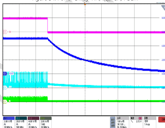
Figure 36. Power Off by EN, I_{OUT}=0A , PFM
