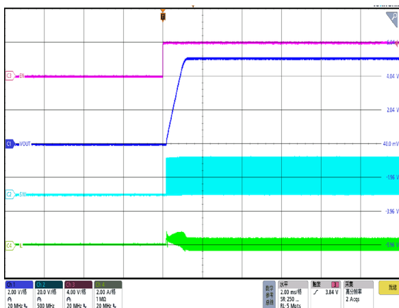
Figure 39. Power On by EN, I_{OUT}=0A , FCCM
