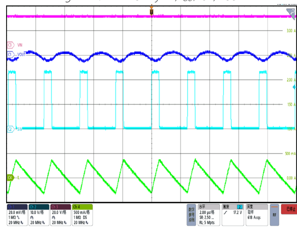
Figure 44. Switching Waveform, I_{OUT}=0A , FCCM
