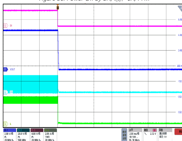
Figure 38. Power Off by EN, I_{OUT}=3A , PFM
