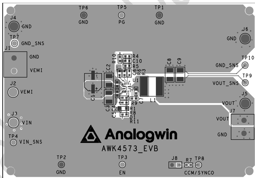
Figure 63. EVM TOP Layer Example
